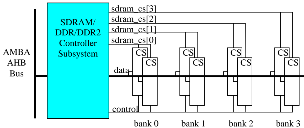
Four SDRAM/DDR/DDR2 SDRAM Banks
