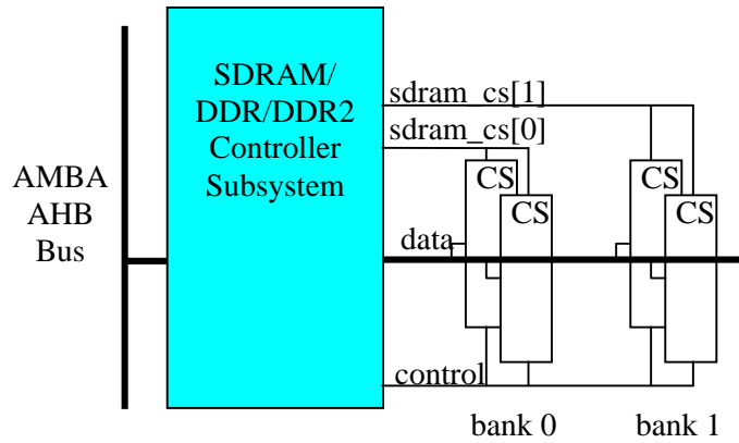
Two SDRAM/DDR/DDR2 SDRAM Banks
